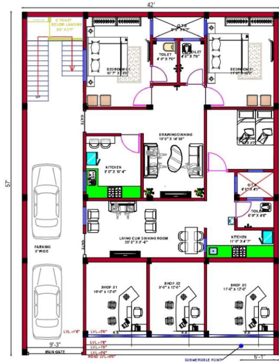
GROUND FLOOR PLAN ----- 12'0" WIDE ROAD -----
