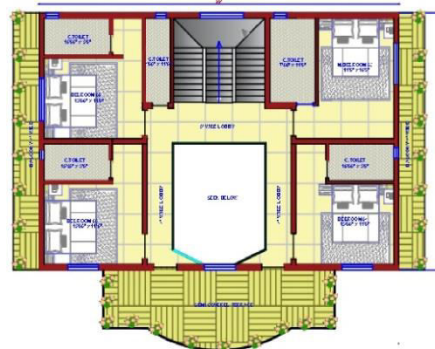
FIRST FLOOR PLAN ---ROAD---
